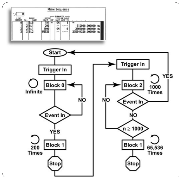
► Figure 40. Pattern generator's sequence flow, showing loops and conditional events.
