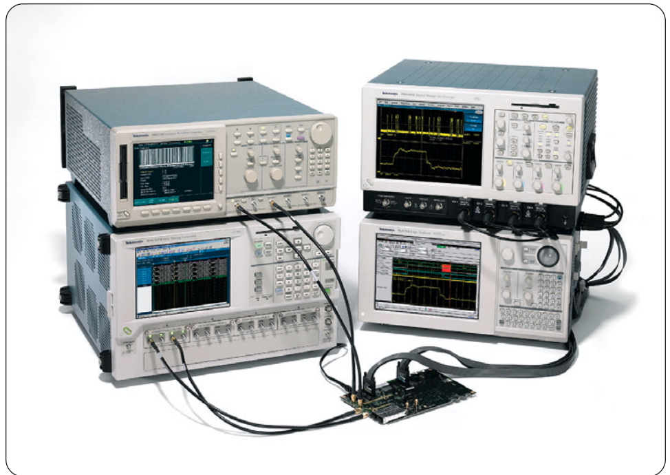
▶ Figure 1. Most measurements require a solution made up of a signal source paired with an acquisition instrument. Triggering connectivity simplifies capturing of the DUT output signal.
