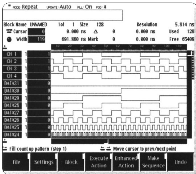
► Figure 41. Multi-channel pattern generator's bus timing display.
