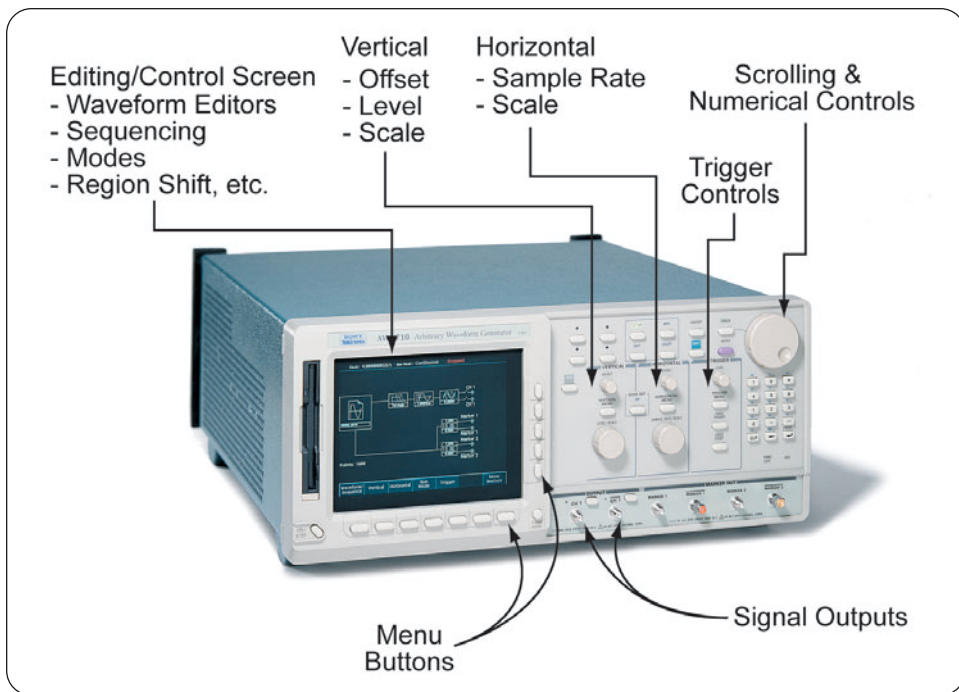
► Figure 18. A high-performance mixed signal source: the Tektronix AWG710 Arbitrary Waveform Generator.
