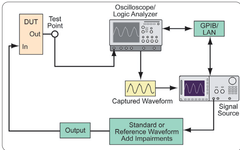
► Figure 3. Signal sources can use standard, user-created, or captured waveforms, adding impairments where necessary for special test applications.
